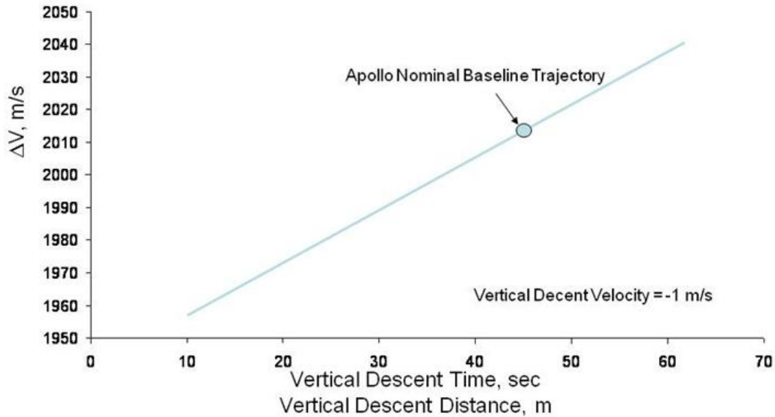
Figure 9. Performance Requirements for Final Vertical Descent.
