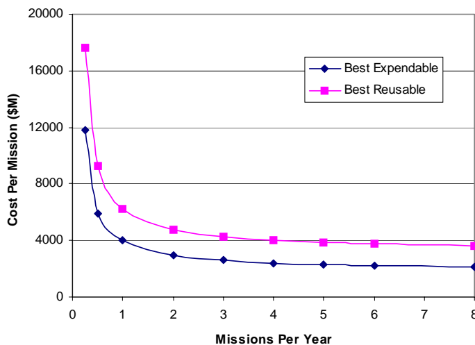
Figure 10: Cost-per-mission as a function of flight rate for the baseline launch vehicle option for the expendable and reusable architectures.
