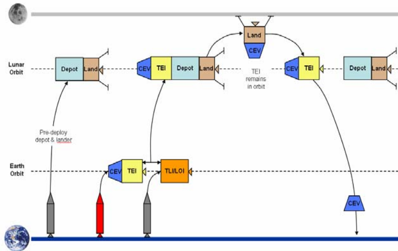
Figure 3. Diagram of Reusable Lunar Architecture.
